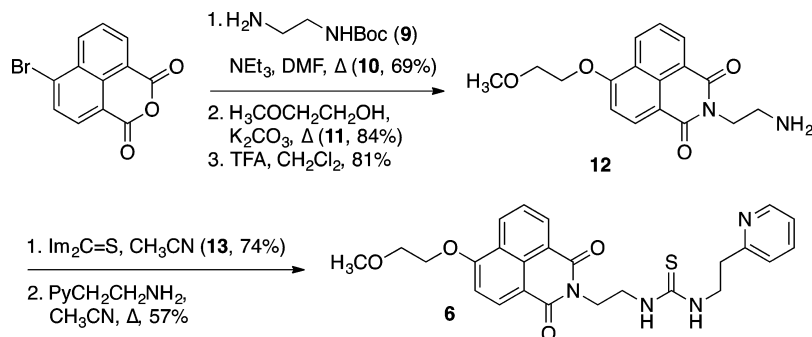
Scheme 1. Synthesis of 6 , a Representative Thiourea (Py = 2-Pyridyl, Im = Imidazolyl) a
