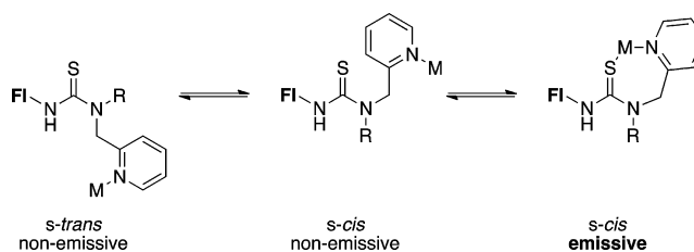
Figure 5. Minimal form of the s-cis/s-trans equilibria in metal complexes of 5 and 7 (Fl = naphthalimide fragment; M = metal ion; R = CH 3 (5), CH 2 Py (7)).
