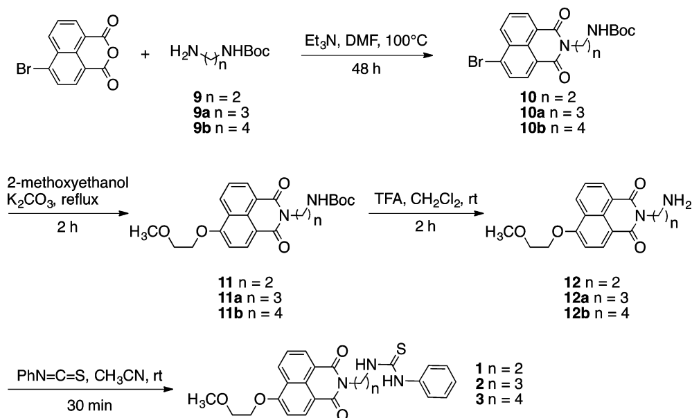
Scheme 2. Synthesis of Phenylthioureas 1–3
